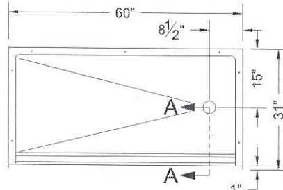
TOP VIEW - SCALE \frac{3}{8}'' = 1'-0''
